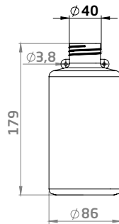
LGM625 Plastic 0,75 L
