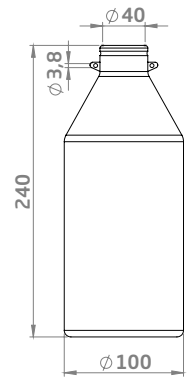
LGM625 Glass 1 L
