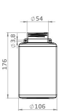
LGM625-L Plastic 1 L
